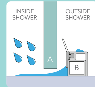
A - Sliding Door Glass B - Minimal Barrier Bar I - Threshold Seal
