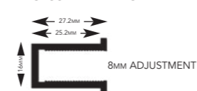
RECESSED WALL CHANNEL PROFILE
